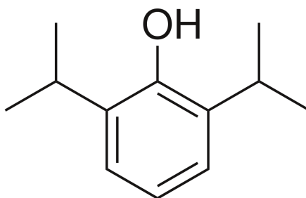
Figure 3.1 – 2,6-diisopropylphenol (propofol).
