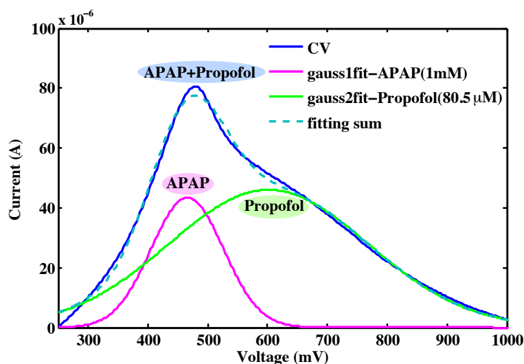
Figure 4.10 – APAP interference study: Gaussian decomposition of the CV procedure ([+0.2 - +1.4] V, scan-rate 0.1 V/s at PGE) belongs to the mixture of APAP (1 mM) and propofol (80.5 \mu M).
