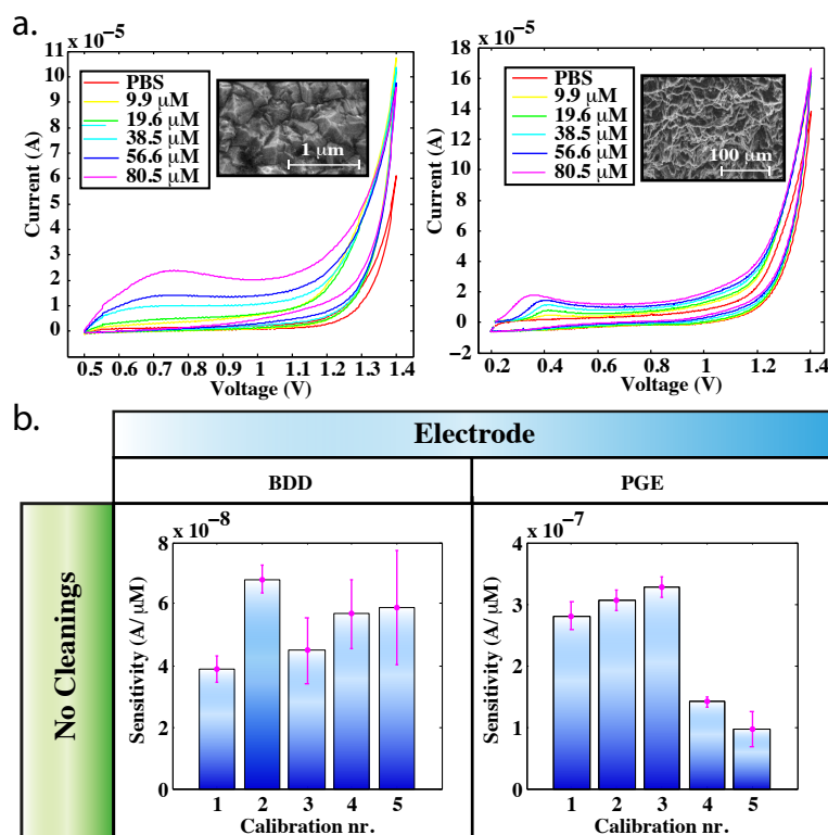
Figure 3.10 – a) Typical CV curves at increasing propofol concentrations ([9.9 - 80.5] \mu M) at PGE and BDD surfaces; (b) change in sensitivity (S) values for BDD and PGE with respect to subsequent propofol calibrations performed in PBS (pH:7.4). Error bars represent the standard deviation from the linear regression analysis performed for S evaluation ( n = 5 , points in each calibration).
