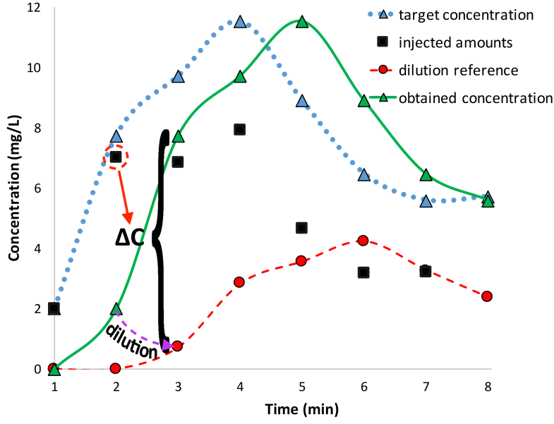
Figure 6.25 – An example of injection dose calculation for reproducing a sample target concentration trend. The baseline dilution is determined for a flow rate of 1 ml/min in a 1 ml base-volume. Differences among the plots have been exaggerated for readability.
