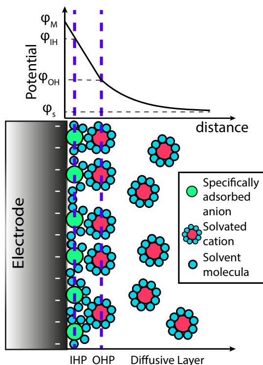
Figure 2.3 – Simplified illustration of the Helmholtz double layer planes where the potential is developed in the area of interface between negatively charged electrode and the electrolyte.
