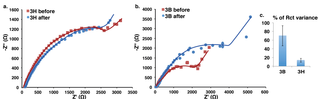
Figure 3.29 – EIS analysis comparison between Not-used and Used PGEs: Nyquist plots of a) 3H and b) 3B, c) bar graph with error bars representing standard error (n = 3) for R_{ct} (%) variance.
