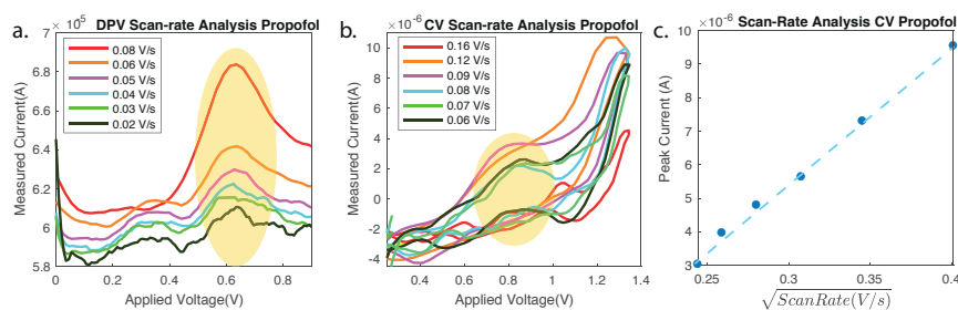
Figure 5.28 – Scan-rate study for 36.5 \mu\text{M} propofol with: a) DPV and b) CV techniques. c) Reports the relationship between scan-rate and oxidation peak current from CV.
