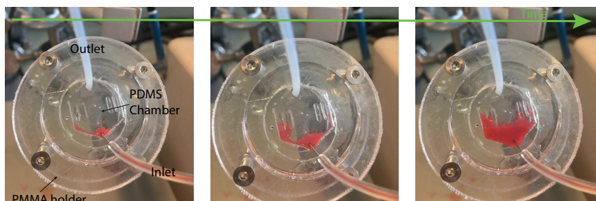
Figure 6.18 – Fluidic chamber tested with red dye flow.
