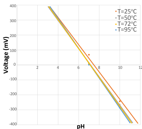
Figure 5.19 – pH calibrations line for different temperatures.
