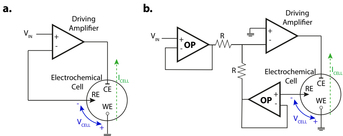
Figure 2.12 – a) General schematic of a grounded WE configuration and b) schematic with voltage buffers to isolate driving amplifier and RE.
