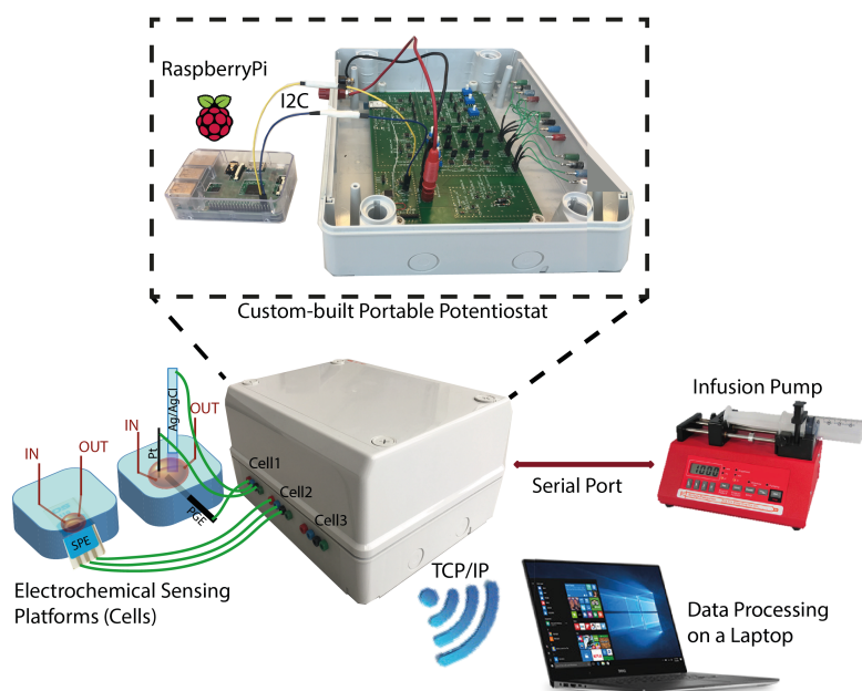
Figure 5.1 – Sketch of the RPi-based portable system for anesthesia monitoring.
