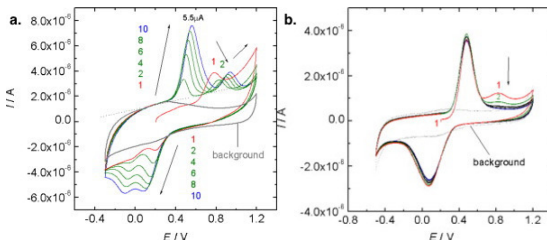
Figure 3.2 – Electrochemical CV characterization of propofol (reprinted from [134]).
