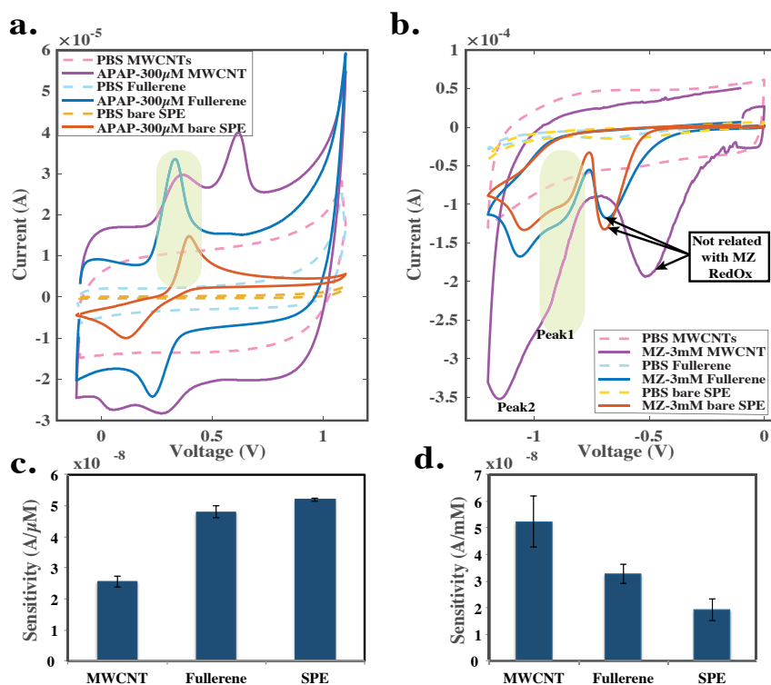
Figure 4.7 – Comparison of voltammograms obtained for: a) APAP 300 \mu M and b) MZ 3 mM at bare, MWCNTs- and fullerene-modified electrodes (PBS blank measurements have been reported for all the electrodes as control). It is visible how nano-structures improve the EASA and electron-transfer properties respect to the bare electrode; c) and d) compares the sensitivity values obtained for the three tested electrodes (calibration performed considering the peaks in the yellow areas).
