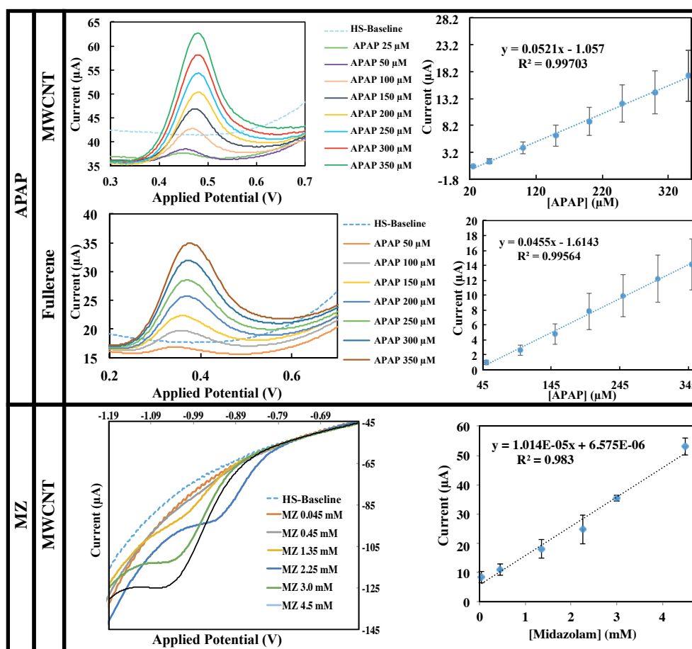
Figure 4.9 – APAP and MZ detection in undiluted HS at MWCNT and fullerene- \text{C}_{60} modified electrodes. Peak areas extracted by the voltammograms and calibration lines ( n = 3 ) are reported for increasing concentrations of APAP and MZ.
