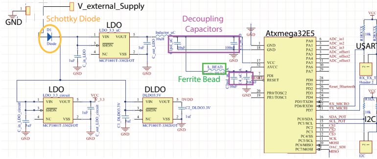
Figure 5.14 – Screen-shot from Altium with the schematic of the microcontroller. The main application notes were respected; e.g. Schottky diode, ferrite beads and decoupling capacitors were included.
