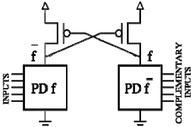
Unipolar DCVSL gate
