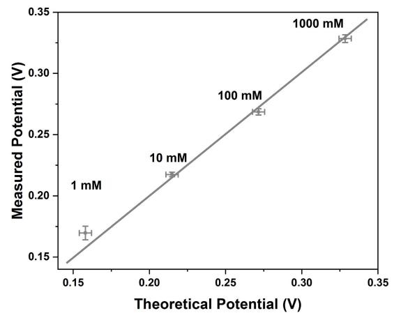
Fig. 8. Comparison between the potential values obtained with the proposed wearable lithium-sensing system with respect to the predicted ones. (X errors are computed using the standard deviation of the calibration curve in sweat, Y errors correspond to different samples of the batch.)
