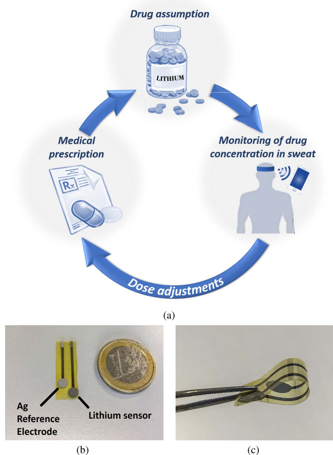
Fig. 1. (a) The principle behind the non-invasive approach proposed in this paper for the Therapeutic Drug Monitoring (TDM) of lithium in sweat. (b) The flexible electrochemical sensing system fabricated in this work for the non-invasive monitoring of lithium. (c) Full bending of the flexible electrochemical lithium-sensing system.
