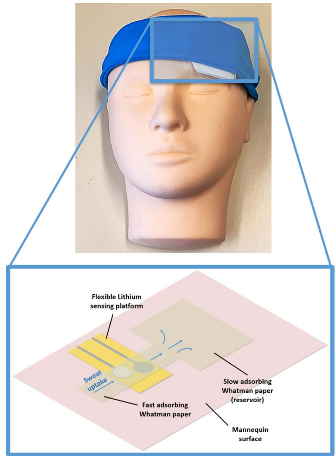
Fig. 7. Experimental setup to simulate in-situ measurements using our wearable lithium-sensing system.
