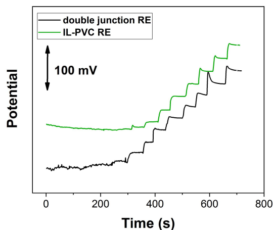
Fig. 4. Calibration time traces recorded with respect to the flexible RE proposed in this work in comparison with a standard Ag/AgCl double junction RE.
