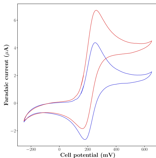
Fig. 8. CV responses at 10 \text{ mV/s} of LOx-C lactate biosensor, in 10 \text{ mM} PBS solution containing 0.5 \text{ mM} HMF: without L-Lactate (blue), with 4.95 \text{ mM} L-Lactate (red).
