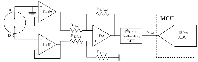
Fig. 5. Circuit architecture for potentiometric readout.
