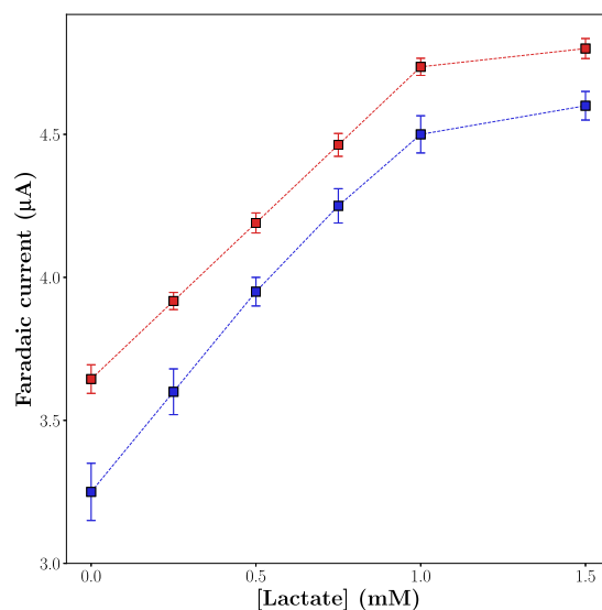
Fig. 9. Calibration curves obtained from CA measurement of LOx-C lactate biosensor at E_{\text{cell}} = 300 \text{ mV} : with AmpPot board (blue), with an Autolab potentiostat (red). The error bars correspond to standard deviations obtained with three measurements, with different sensors.
