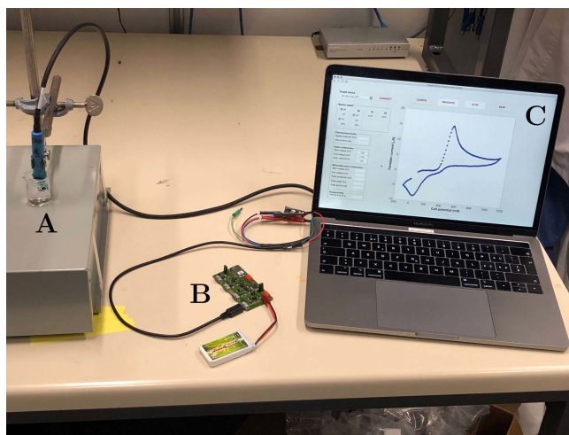
Fig. 1. System setup for in-vitro characterization of paracetamol: A Carbon screen-printed electrode in a solution of PBS and controlled concentration of paracetamol; B hardware front-end powered by Li-ion battery; C GUI to configure the measurements and to acquire voltammograms.
