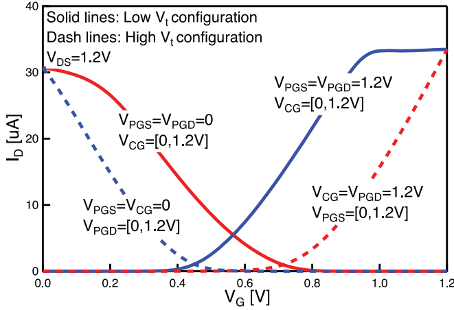
Fig. 8. Simulated triple-independent-gate vertically stacked nanowire transistor characteristic.
