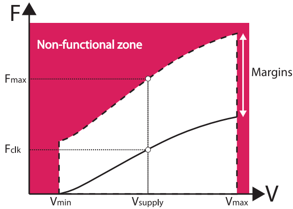
Fig. 18. VF functional domain and design margins.
