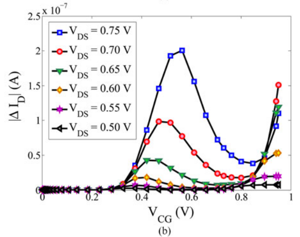
Fig. 6. Difference of I_D with and without GOS under CG versus V_{CG} . (a) Samples of |\Delta I_D| - V_{CG} for V_{DS} \geq 0.8 . The curves can be modeled by a degree-2 polynomial above the threshold. (b) Samples of |\Delta I_D| - V_{CG} for V_{DS} \leq 0.8 . The curves can be modeled by a degree-3 polynomial above the threshold.
