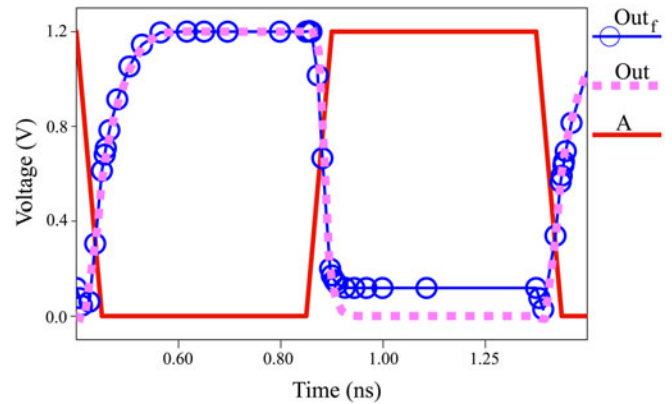
Fig. 8. GOS occurrence in CG of the pull-down transistor of an Inverter.
