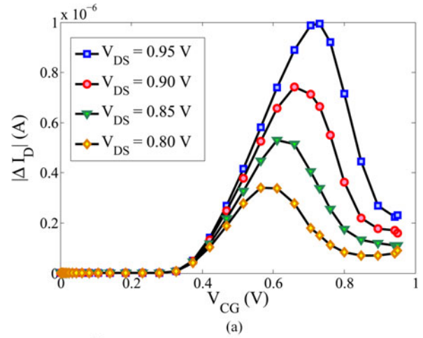
Fig. 4. Behavior of defective n-type TIG-SiNWFETs in the presence of GOS: (a) GOS under PG_S , (b) GOS under CG , and (c) GOS under PG_D .
