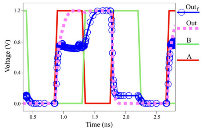
Fig. 9. GOS occurrence in CG of a pull-down transistor (t3) of an XOR.
