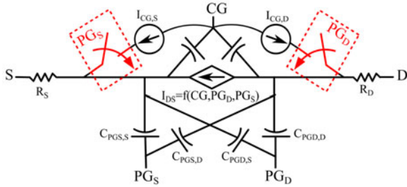
Fig. 5. Nonlinear piecewise model of GOS under CG for n-type TIG-SiNWFETs. The switches are necessary to realize the impact of the PGs on the leakage of defective device in DP logics.
