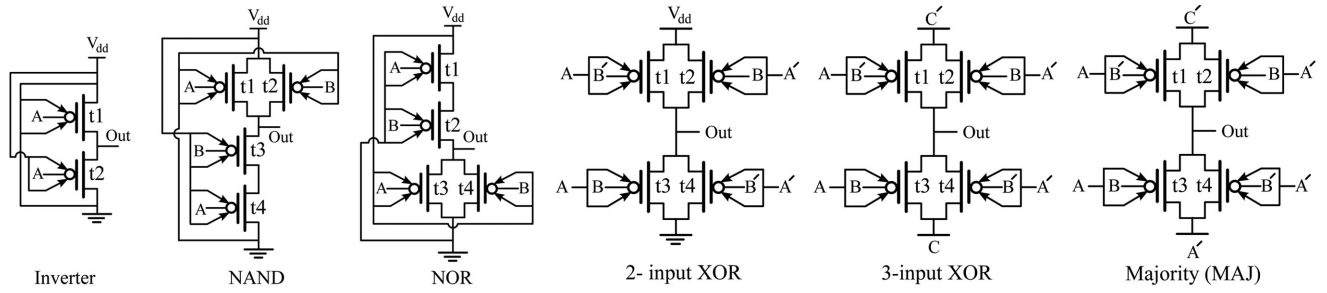
Fig. 2. Logic gate realization in TIG-SiNWFET. Inverter, NAND, and NOR gates are the examples of the SP logic gates. Accordingly, 2-input XOR, 3-input XOR and MAJ logic gates are those of DP logic structures.
