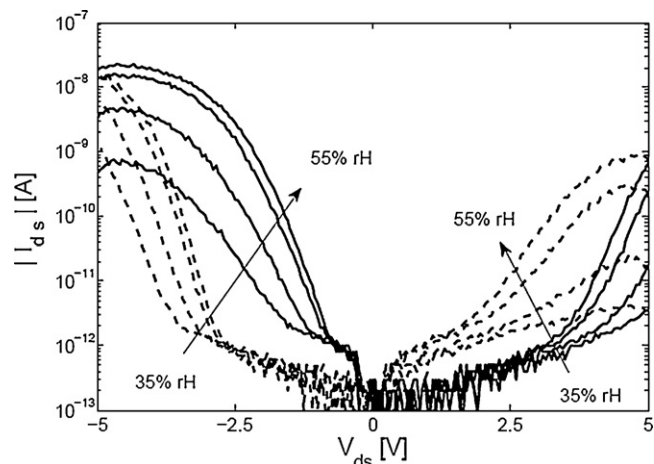
Fig. 13. Effect of increasing air humidity on the I_{ds} - V_{ds} curves taken at T = 22 °C. The curves are taken within a 40 min time frame and follow an humidity gradient induced by inserting a water tank inside the measurement chamber. Continuous sweeps taken every 10 min confirm the increase of current upon increasing air humidity levels along with rH saturation at 55%.
