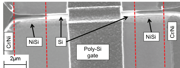
Figure 4. GAA SiNW SBFET with Cr/Ni source/drain after the lift-off process. The change in contrast on the NW channel is attribute to a difference between Si and silicided regions.
