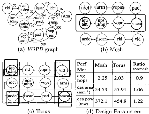
Figure 3: Example Mappings of VOPD
