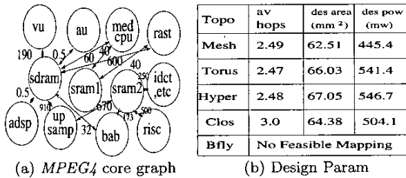
Figure 7: MPEG4 Mappings
