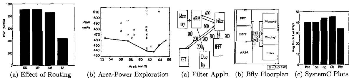
Figure 9: Design Space Exploration of a Topology
