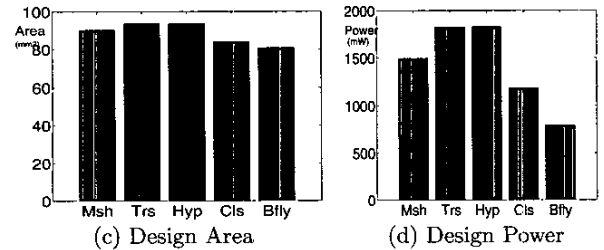
Figure 8: Network Processing Application
