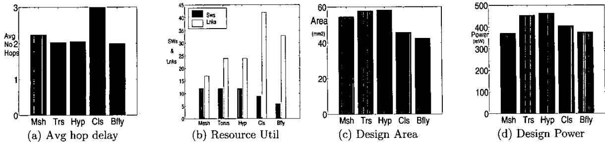
Figure 6: Mapping Characteristics of VOPD
