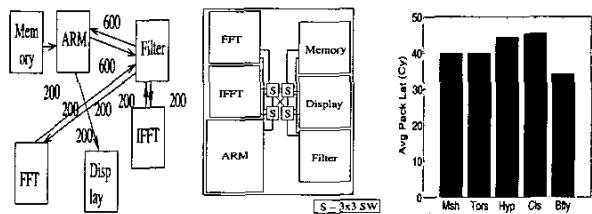
Figure 10: Mapping of DSP Application
