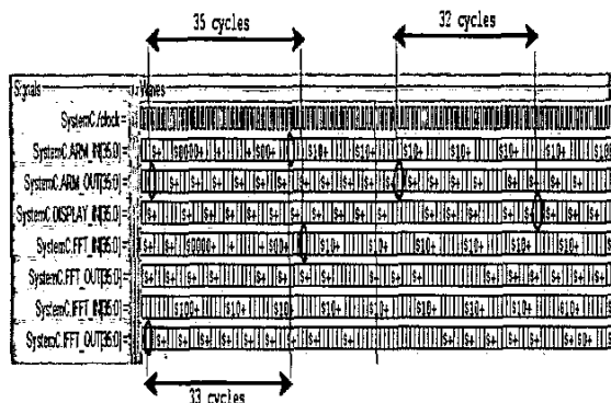
Figure 11: SystemC Snapshot
