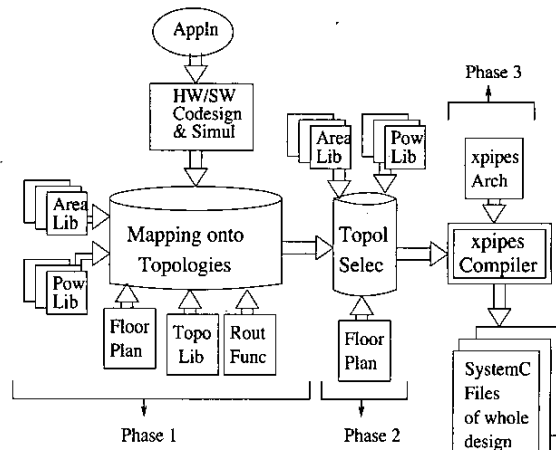
Figure 4: Design Flow of SUNMAP
