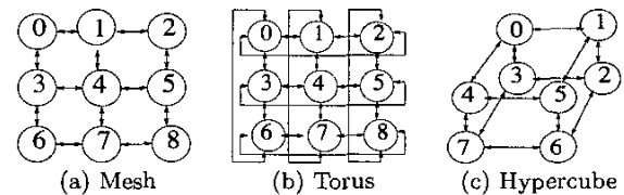
Figure 1: Direct NoC Topologies
