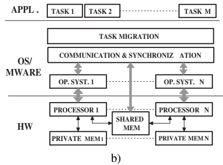
Figure 3: a) Target hardware architecture; b) Scheme of the software abstraction layer.
