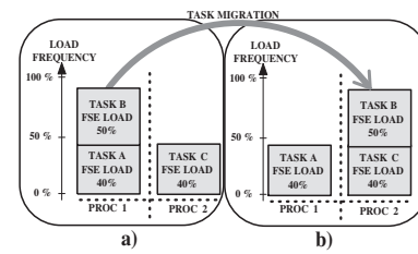
Figure 1: Simple thermal balancing example
