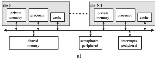
Figure 3: a) Target hardware architecture; b) Scheme of the software abstraction layer.
