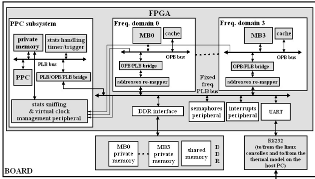
Figure 1: Overview HW architecture of emulated MPOS MP-SoC platforms
