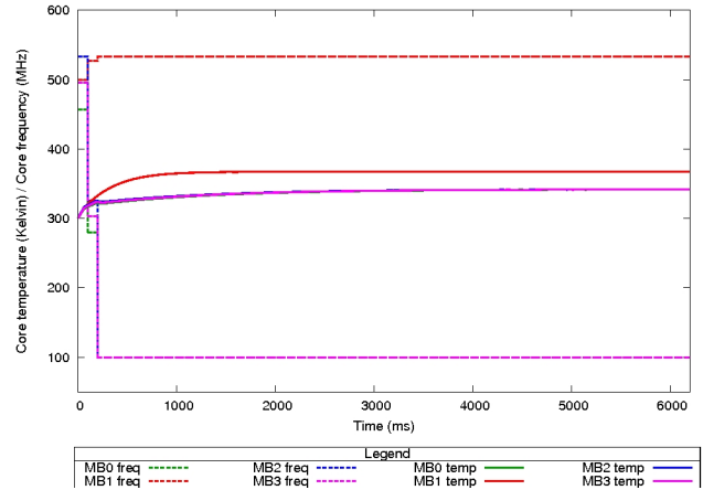
Figure 5: Temperature waveform with one task running on MB1
