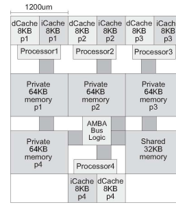
Figure 4: MPSoC floorplan with uneven distribution of cores on the die and a shared bus interconnect
