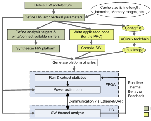
Figure 3: Complete HW-SW flows included in the FPGA-based thermal emulation framework
