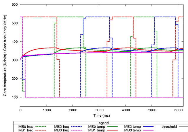
Figure 6: Temperature effect of a simple temperature-aware task migration policy.
