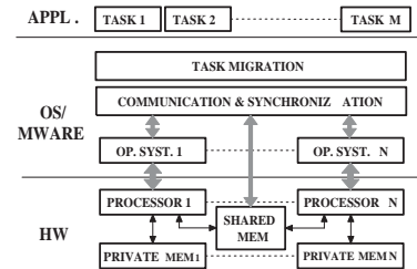
Figure 2: Scheme of the software abstraction layer
